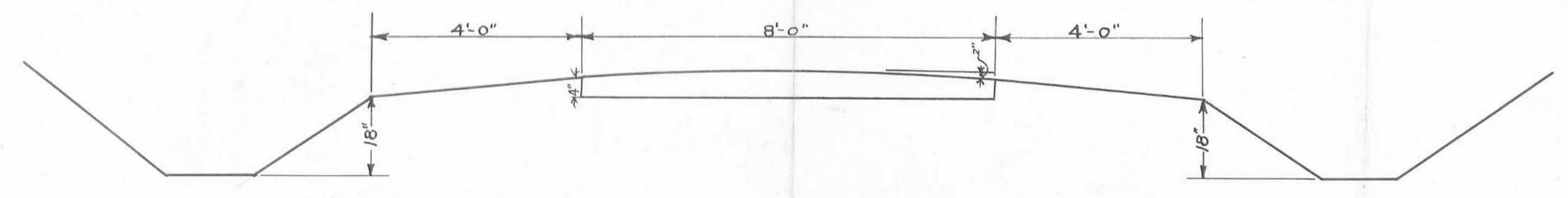
CROSS Section
