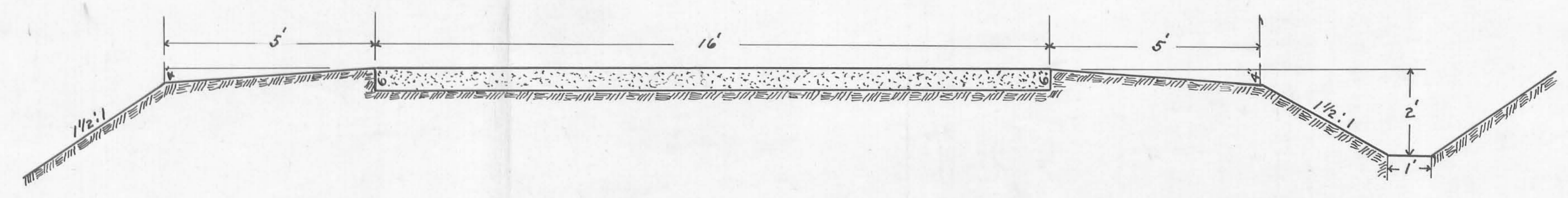
CROSS SECTION
