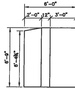
DETAIL PLAN OF PRE-CAST WINGWALL TYP. OF 2 CORNERS BUILT @ 10° FLARE
